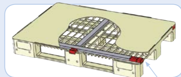
Reinforced pallet
